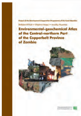
Environmental- geochemical Atlas of the Central- northern Part of the Copperbelt Province of Zambia, slož. v obálce 260,-
